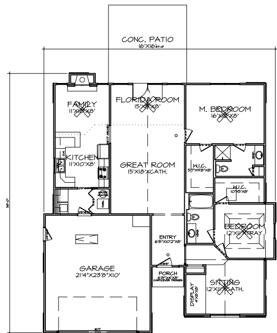
1 FIRST FLOOR PLAN A-4
