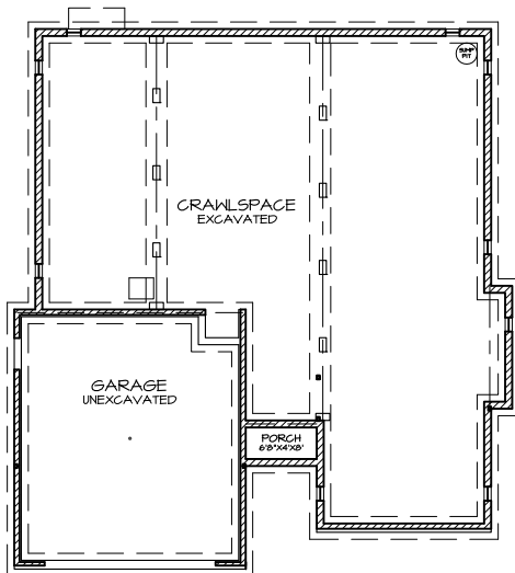
1 FOUNDATION PLAN A-3
